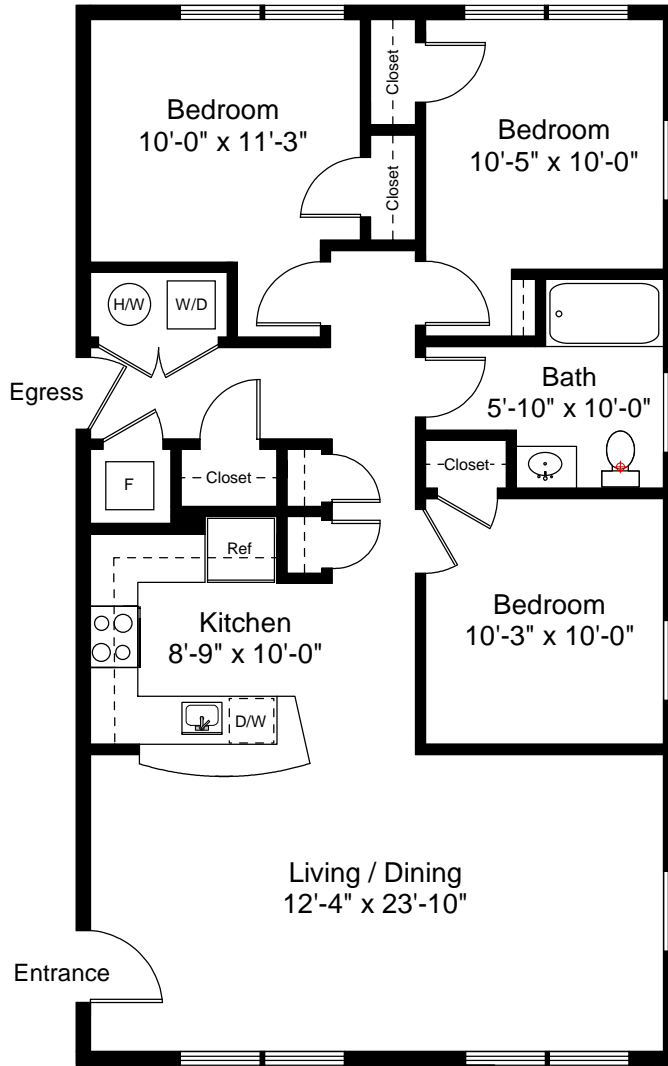
Typical Floor Plan - Units 3, 9, 7, 13 Ceiling Height = 8'-6"
